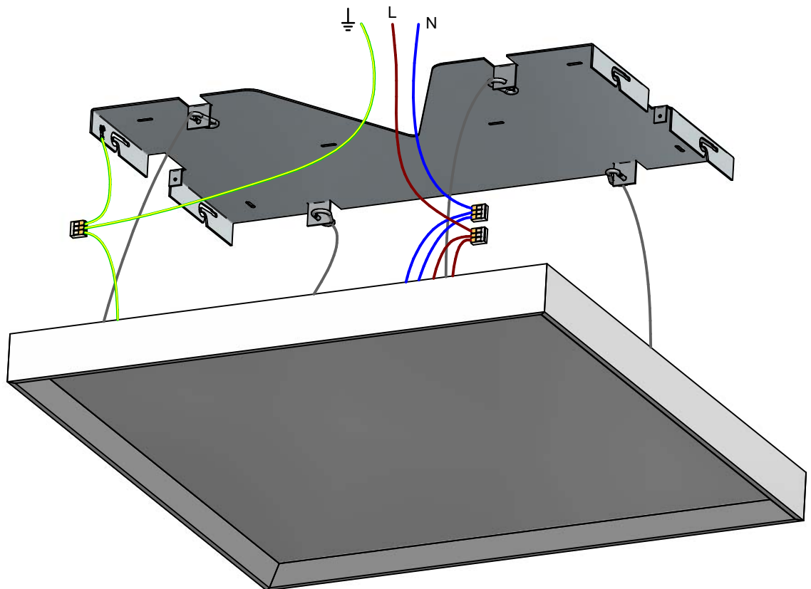
KIT0026 Dimmer NOT INCLUDED
